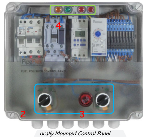
Locally Mounted Control Panel
