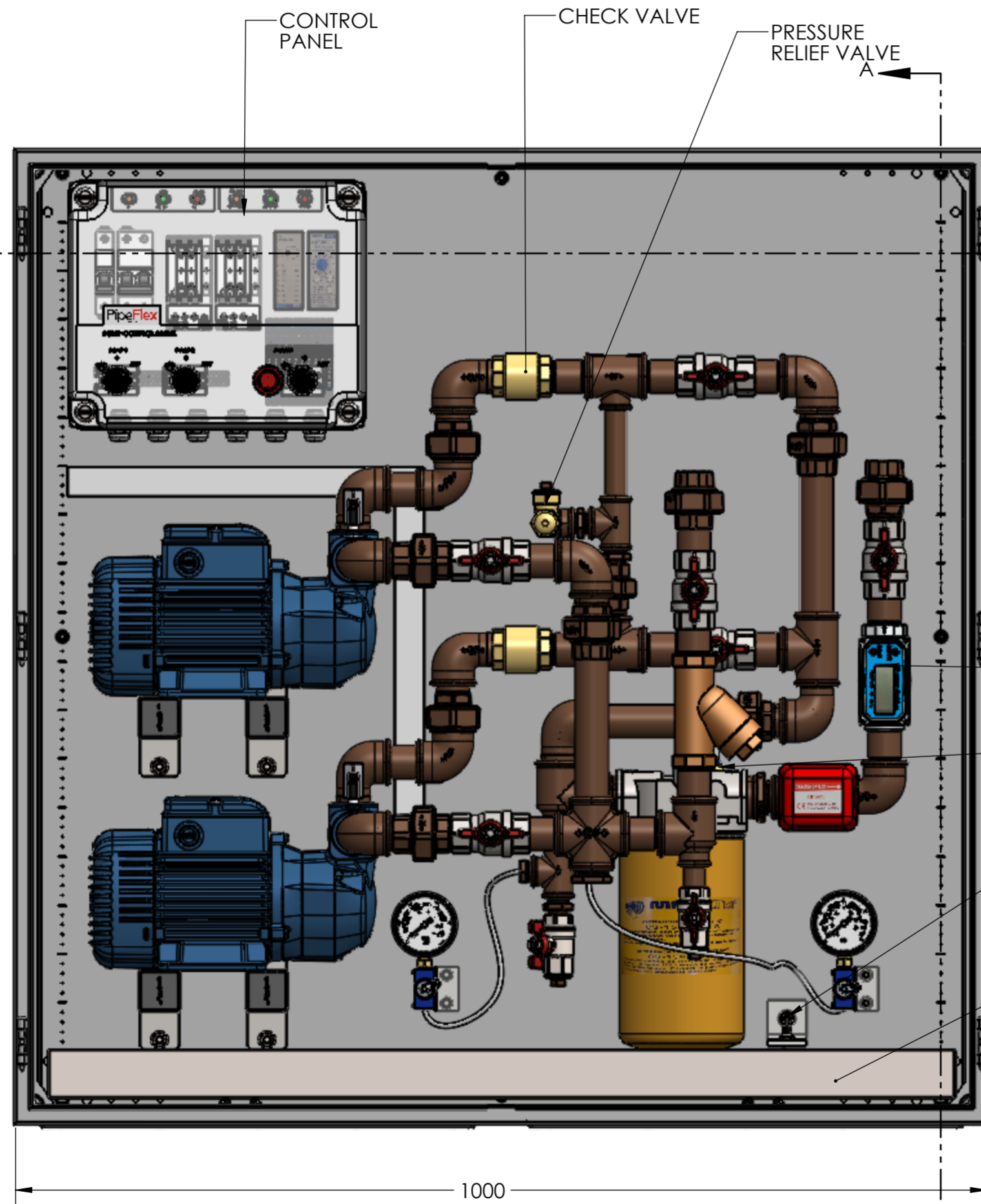
VIEW ON PUMP SET (ENCLOSURE DOORS OMITTED FOR CLARITY)
